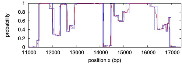
FIG. 9. (Color online) The probability profile 1-p_{\text{bp}}(x) of Fig. 7 is plotted here (in red) with its upper and lower bounds (in blue), 1-p_{\text{low}}(x) and 1-p_{\text{up}}(x) , obtained from the stitch profile.
