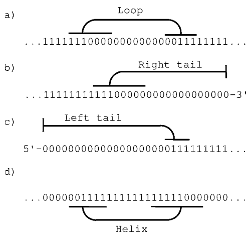
FIG. 1. A stitch profile is composed of four types of stitches: (a) loops, (b) right tails, (c) left tails, and (d) helices. Loop and tail stitches are drawn on the upper side and they span regions of opened base pairs (0’s). Helix stitches are drawn on the lower side and they span regions of closed base pairs (1’s). The horizontal bars indicate fluctuational ranges of the 0-1 boundaries.
