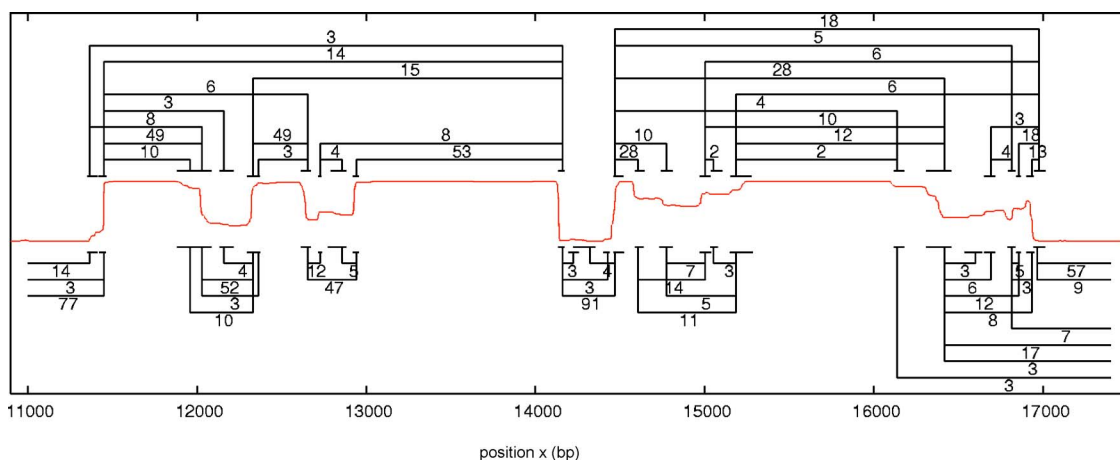
FIG. 7. (Color online) Comparison of a stitch profile and a probability profile, both calculated at T\approx 90^\circ\text{C} where the helicity is \Theta=0.1 . The curve in the middle (in red) is the probability profile 1-p_{\text{bp}}(x) and it varies between 0 and 1 (vertical axis not shown). Each stitch is labeled with its peak volume p_v in percent. The parameters are D_{\max}=3 and p_c=0.02 and the sequence window is 11–17.4 kbp.
